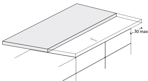
b. Protruding version
